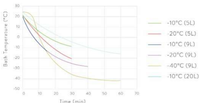
Cooling Curve Bath Liquid: Ethanol
