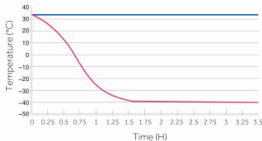
FSF-40V328E Pull Down Test at Ambient 32°C
